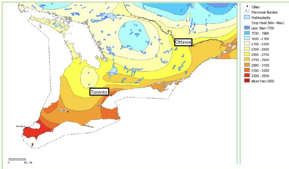
Figure 2: Marginal class 3 lands and zones of 2100-2700 CHU are optimal target areas for switchgrass production in Ontario, Canada. (2)
